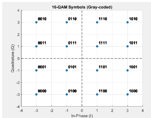
Figure 10: 16-QAM Constellation
