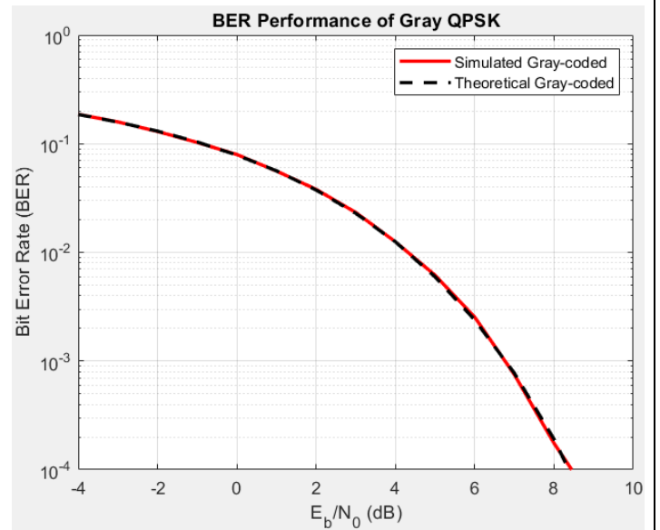
Figure 14: BER of Gray coded QPSK
