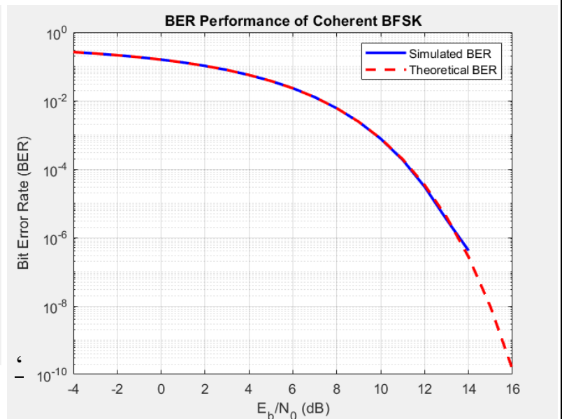
Figure 46: BER of BFSK
