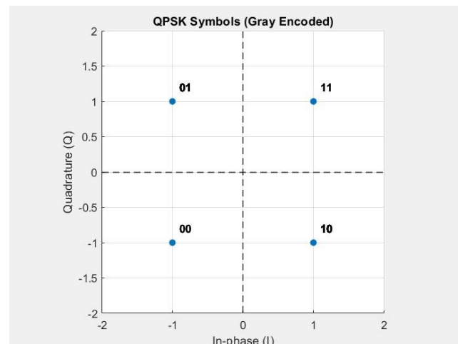
Figure 3: QPSK Gray Constellation
