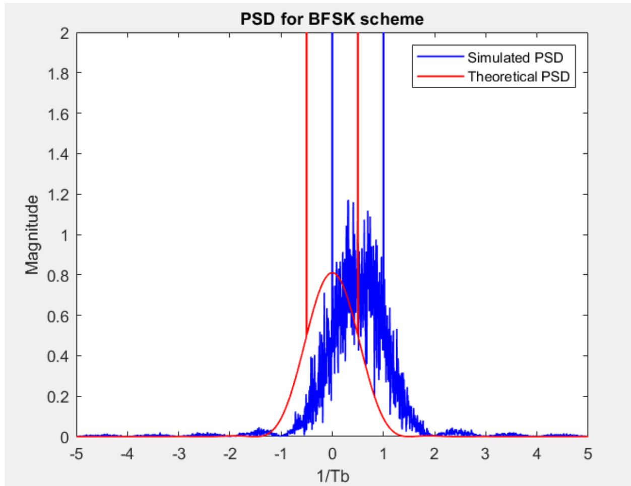
Figure 50: PSD for BFSK
