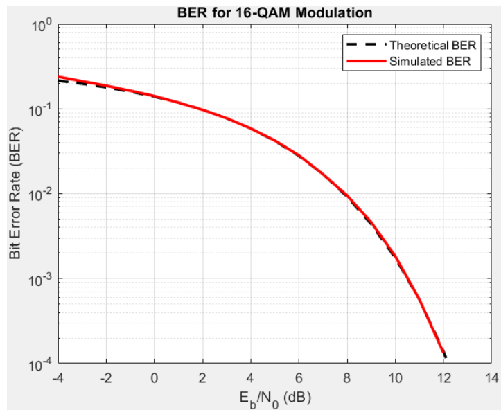
Figure 33: BER of 16-QAM
