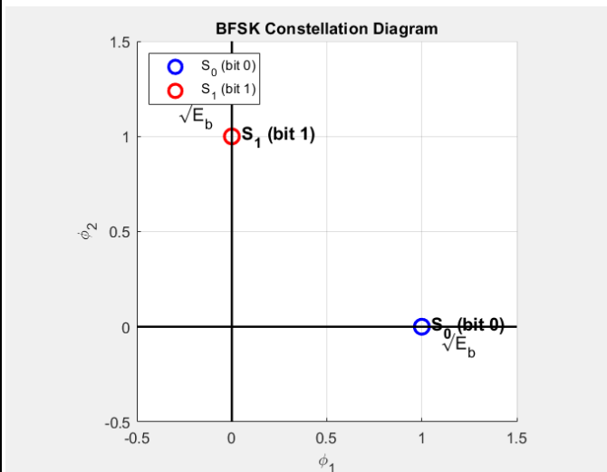
Figure 45: BFSK Constellation
