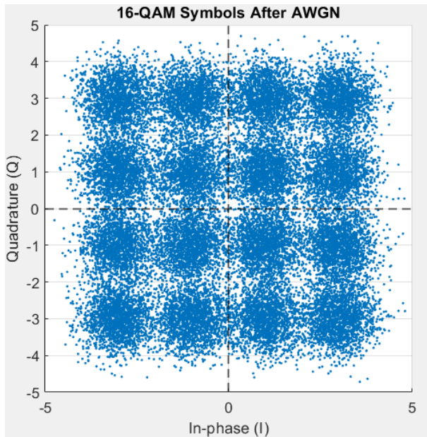
Figure 19: 16-QAM symbols after AWGN at SNR = 5
