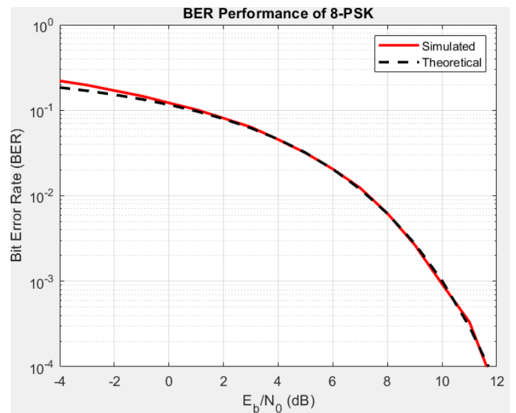
Figure 16: BER of 8-PSK
