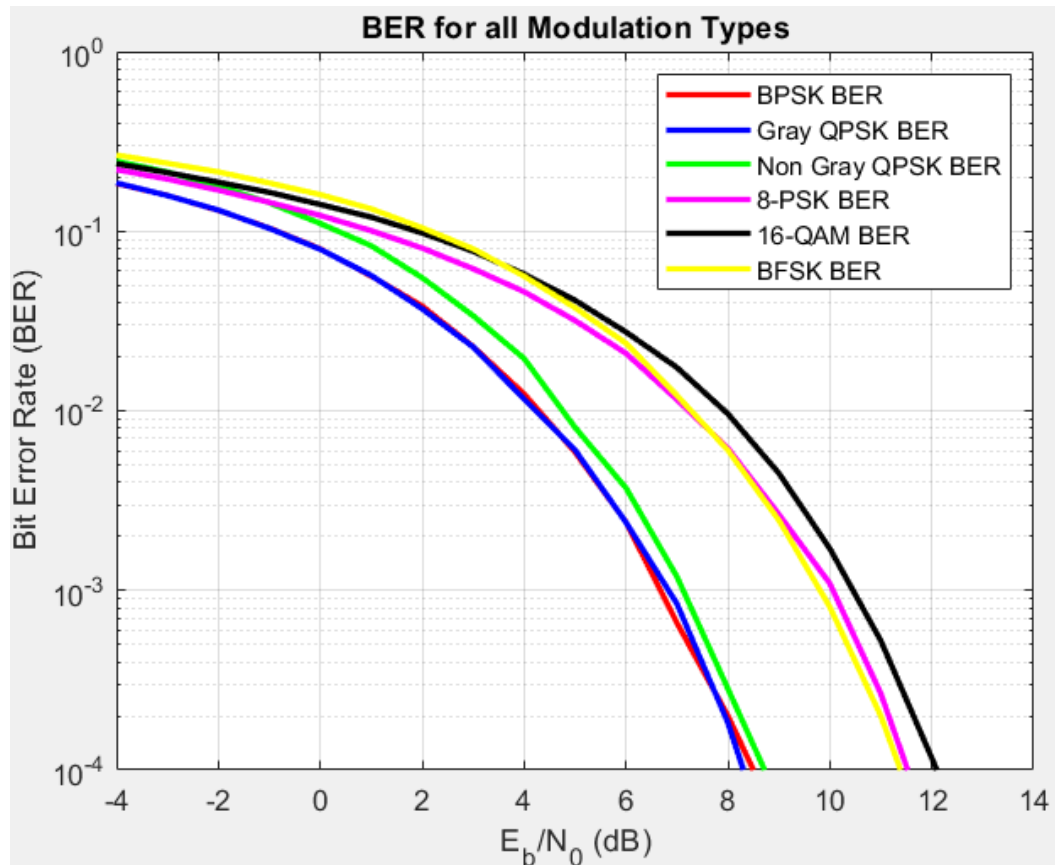
Figure 41: BER for all modulation types
