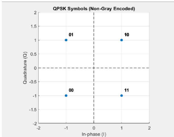
Figure 4: QPSK Non-Gray Constellation
