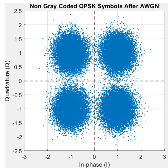
Figure 10: Non-Gray coded QPSK after AWGN at SNR = 5
