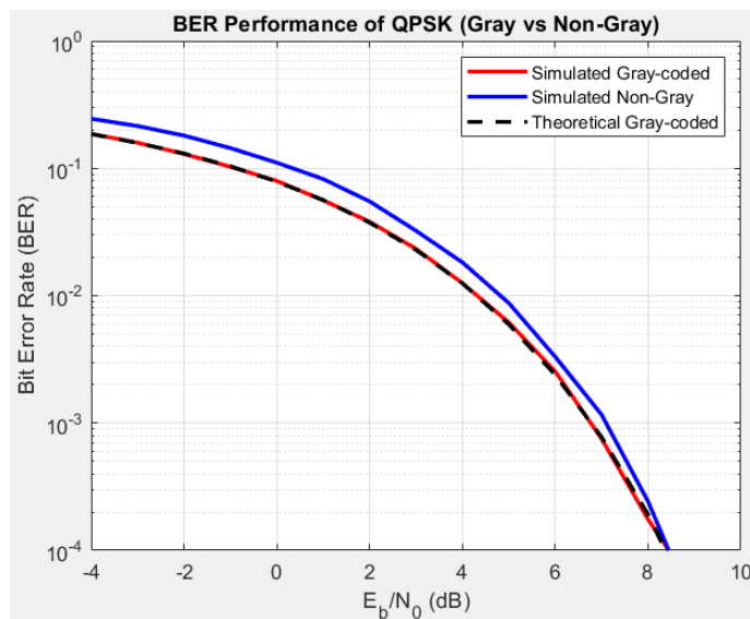
Figure 15: BER of Non-Gray coded QPSK
