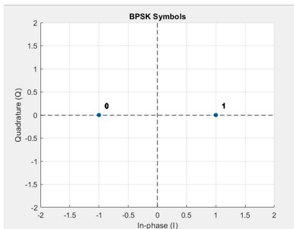
Figure 2: BPSK Constellation
