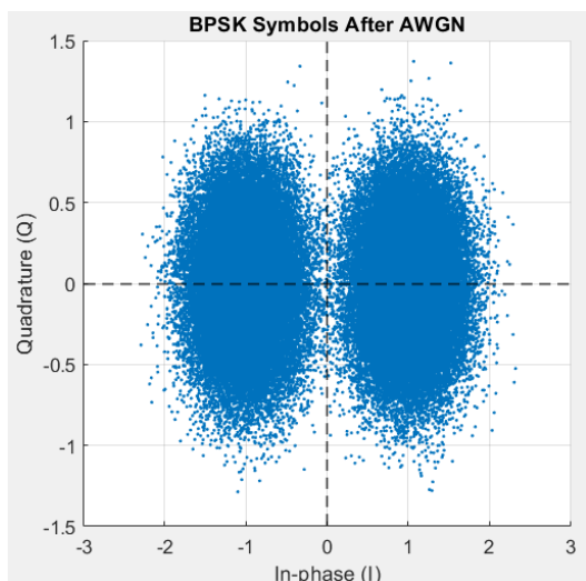
Figure 7: BPSK symbols after AWGN at SNR = 5
