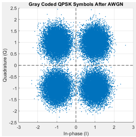
Figure 9: Gray coded QPSK after AWGN at SNR = 5
