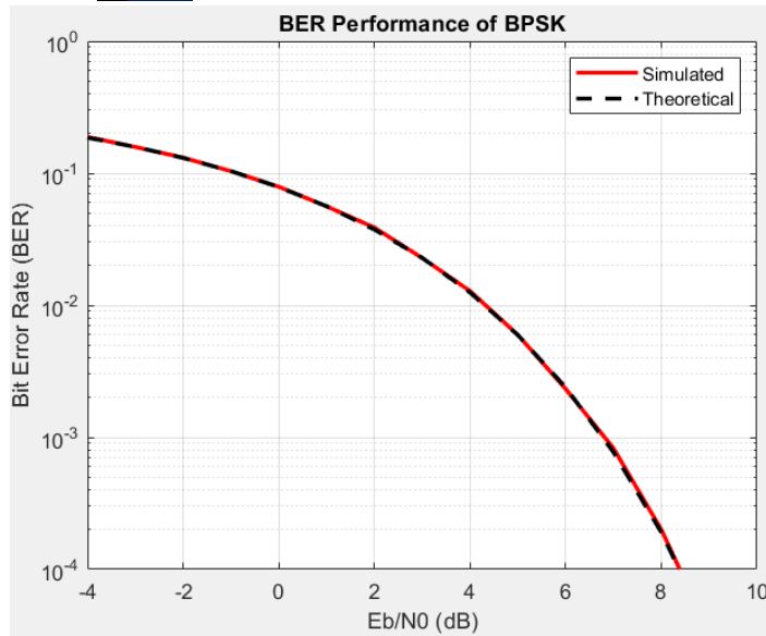
Figure 3: BER of BPSK
