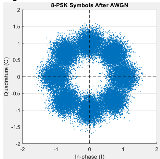
Figure 8: 8-PSK symbols after AWGN at SNR = 5
