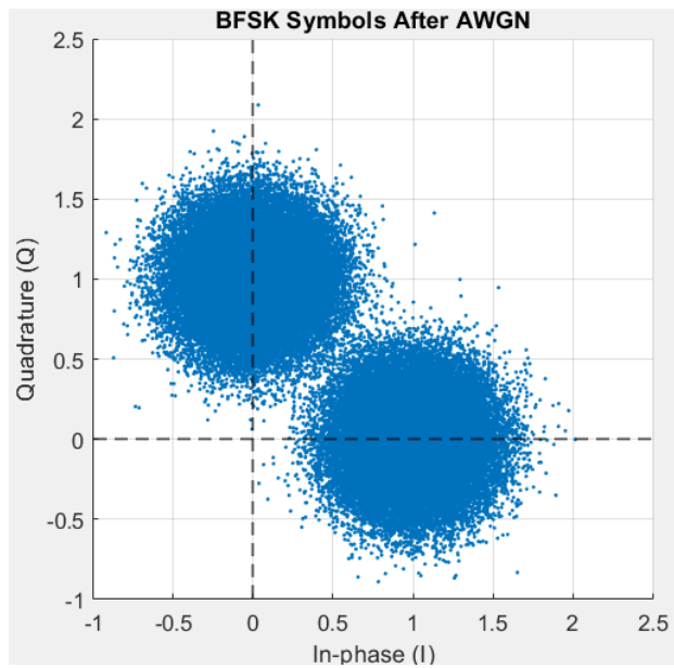
Figure 15: BFSK symbols after AWGN at SNR = 10
